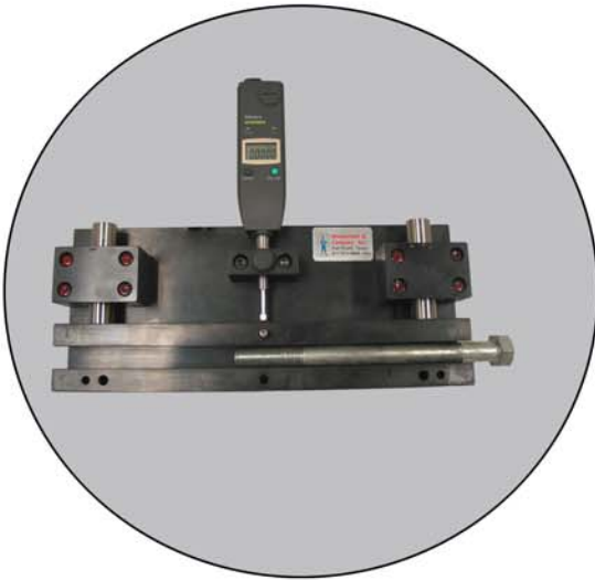
Step 1 - Zeroing the gage
