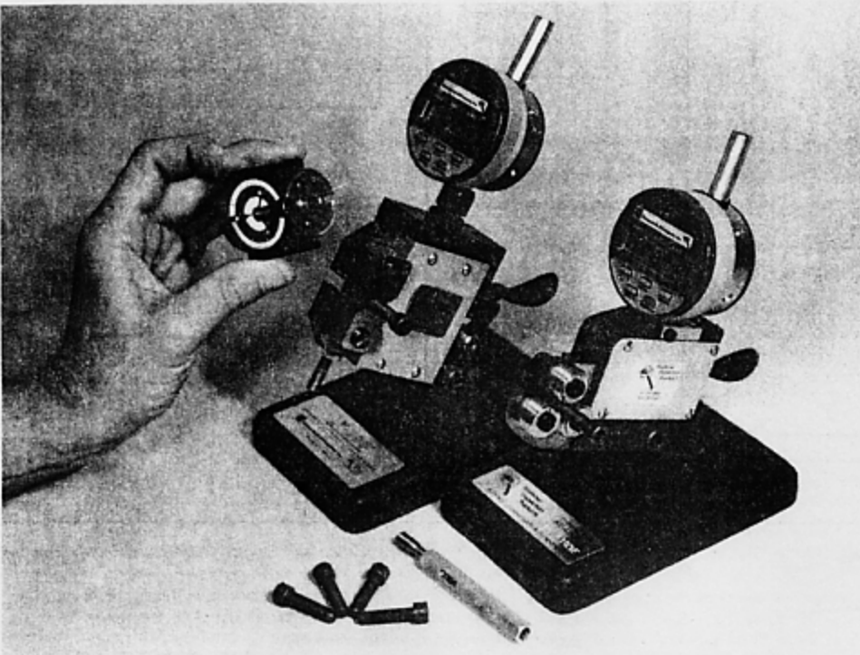
Ring gage, segment gage, and tri-roll gages are all permissible gages for measuring "functional diameter" per ANSI/ASME B1.3-1986.
